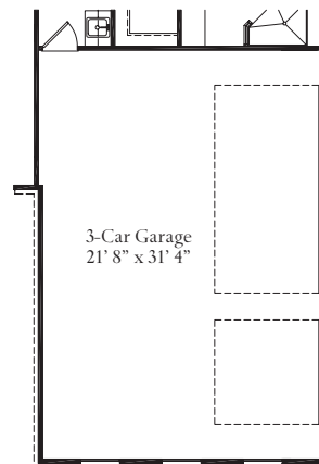
Partial main level with opt. 3-car side load garage
