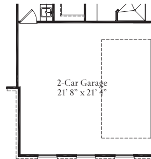
Partial main level with opt. 2-car side load garage
